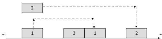
Fig. 10. Event generation in event-driven model
