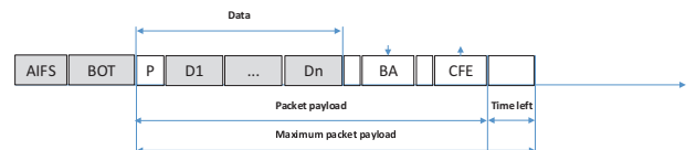
Fig. 4. BASIC signaling
