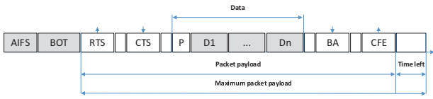
Fig. 5. RTS/CTS signaling
