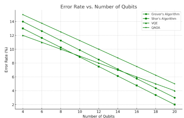
Fig. 4. Error Rate Distribution Across Quantum Algorithms for Increasing Qubit Numbers
