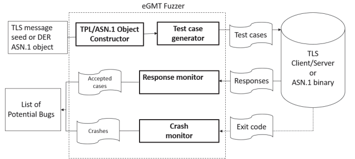
Fig. 3. eGMT-Fuzzer components
