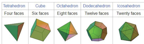
Fig. 6. Five Platonic solids – convex, regular polyhedrons in three-dimensional Euclidean space
