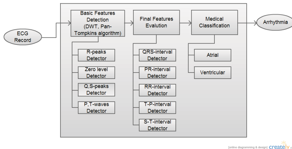
Fig. 2. Main algorithm
