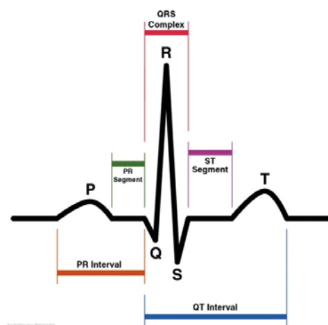
Fig. 1. Electrocardiogram
